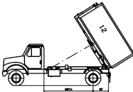
MAX. DUMPING ANGLE 58 DEG
