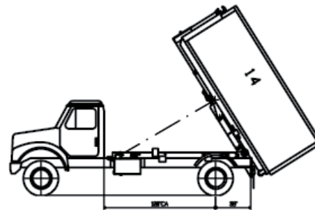
MAX. DUMPING ANGLE 58 DEG
